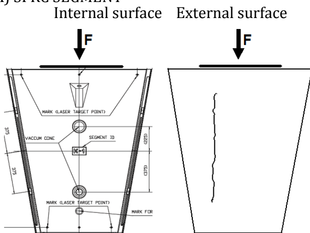
Figure 6. Record of macrocrack location - SFRC key segment - F_{fc,cr} = 4200\text{kN}
