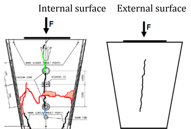
Figure 9. Record of macrocrack location under maximum load - RC segment - F_{fc,u} = 5868\text{kN}
