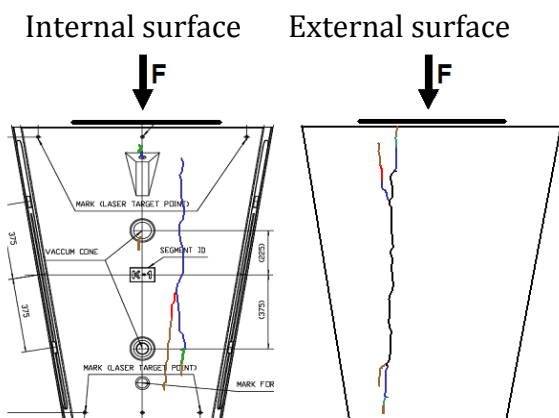
Figure 7. Record of macrocrack location under maximum load
