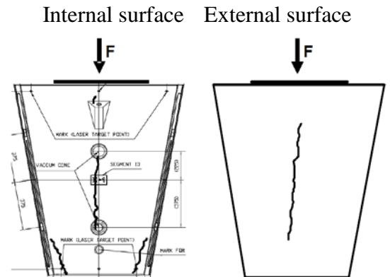
Figure 8. Record of macrocrack location - RC segment - F_{fc,cr} = 3300\text{kN}
