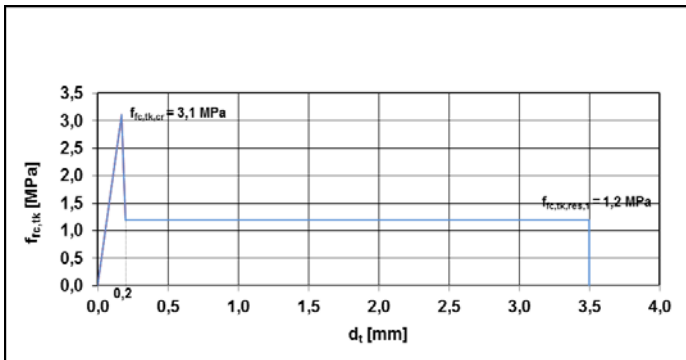
Figure 3. Example of stress-strain diagram ( f_{fc,tk} - \delta_{t,i} ) i.e. (char. Central tensile strength – deflection) using simplified diagram
