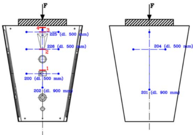
Figure 5. The test arrangement including locations of potentiometers and tensometers
