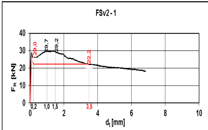
Figure 1. Stress-strain diagram
