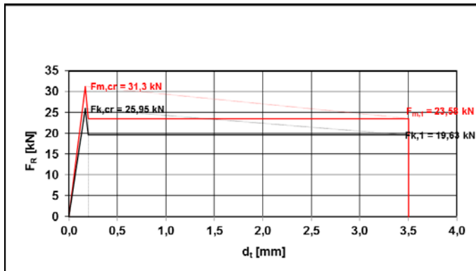
Figure 2. Simplified idealised stress-strain diagrams: average, characteristic
