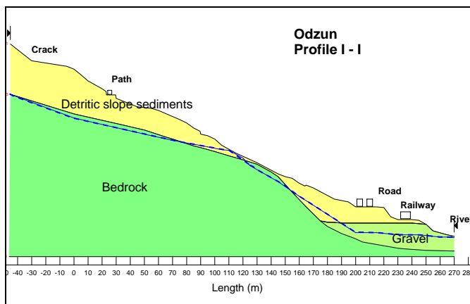
PROFILE OF THE LANDSLIDE AREA
