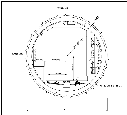
CROSS SECTION 1 – RUNNING TUNNELS (TBM)
