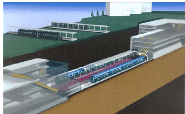
“FÖVAM TER” STATION - COMPUTER SIMULATION
