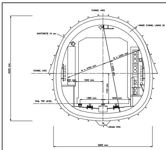
CROSS SECTION 2 – RUNNING TUNNELS (NATM)
