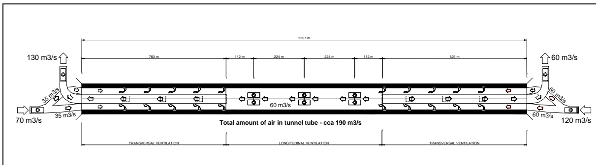
VENTILATION SCHEME
